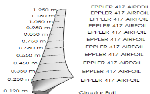
Figs (27) combination between lift/drag twist opt and Betz chord opt.
