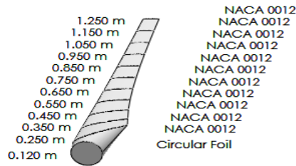
Fig. (38) Combination between lift/drag Twist opt and Schmitz chord opt.
