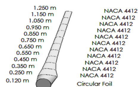
Fig. (29) Combination between none Opt Twist opt and Schmitz chord opt.
