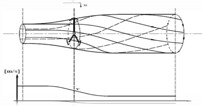
Figure (6) Downstream Rotation of the Wake
