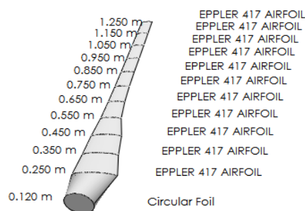
Fig. (23) Combination between none twist opt and Schmitz chord opt.
