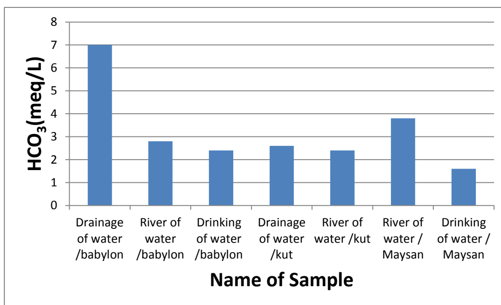
Fig. (9) Bicarbonates levels for studied water samples
